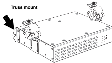
Figure 3: Mounting options
